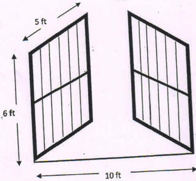
Specification and design of Farm gate size 5' x 10'
